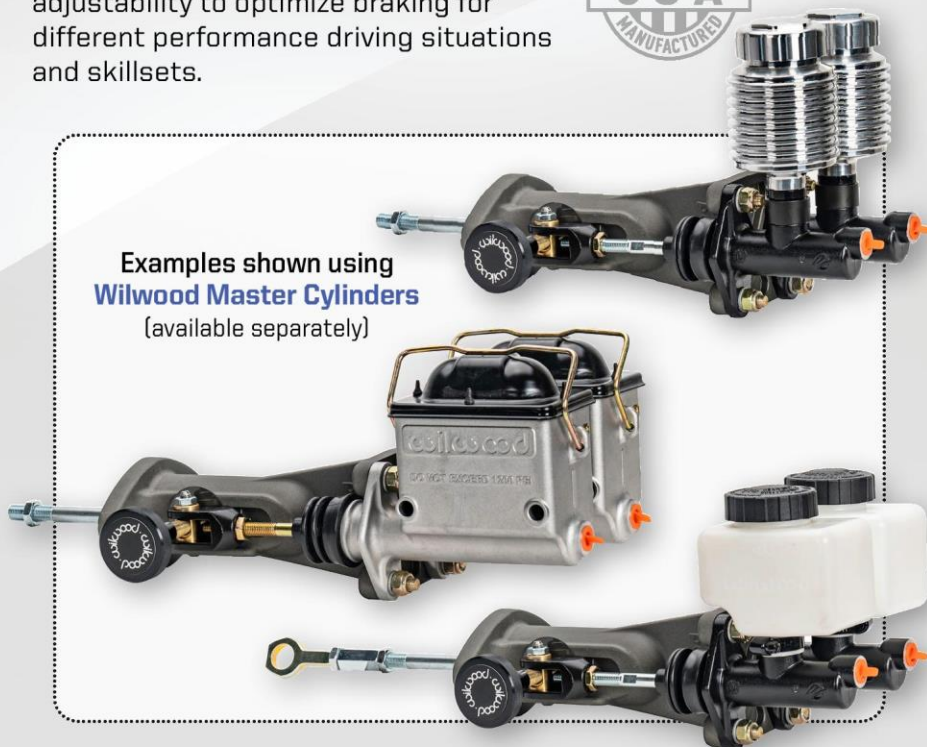
Tandem Mount Balance Bar Assembly with Eyelet
